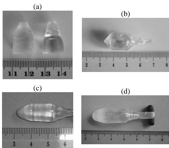
Fig. 1. Y_{1-x}R_xCa_4O(BO_3)_3 as-grown crystals: (a) Y_{0.8}Lu_{0.2}Ca_4O(BO_3)_3 and Y_{0.6}Lu_{0.4}Ca_4O(BO_3)_3 crystals, (b) Y_{0.7}Lu_{0.3}Ca_4O(BO_3)_3 crystal, (c) Y_{0.8}Sc_{0.2}Ca_4O(BO_3)_3 , (d) Y_{0.7}Sc_{0.3}Ca_4O(BO_3)_3 crystal.
