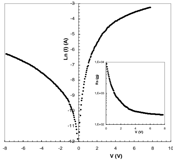
Fig. 1. The semi-logarithmic \ln I - V characteristics of the (Ni/Au)/AlGaIn/GaN heterostructure.
