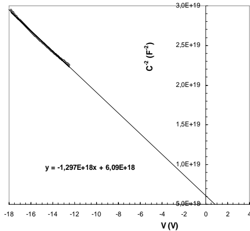
Fig. 6. The C^2 - V plot for (\text{Ni}/\text{Au})/\text{AlGaN}/\text{GaN} heterostructure.
