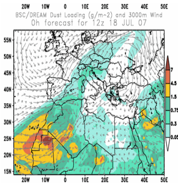
Fig. 2. Saharan dust distribution in Romania and Greece, 17-18 July 2007.
