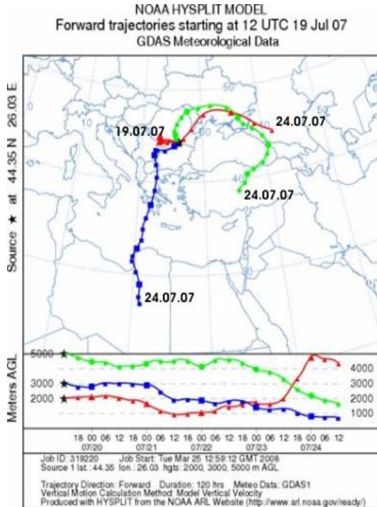
Fig. 14. Air mass forward-trajectories from Romania, on 19 July 2007.
